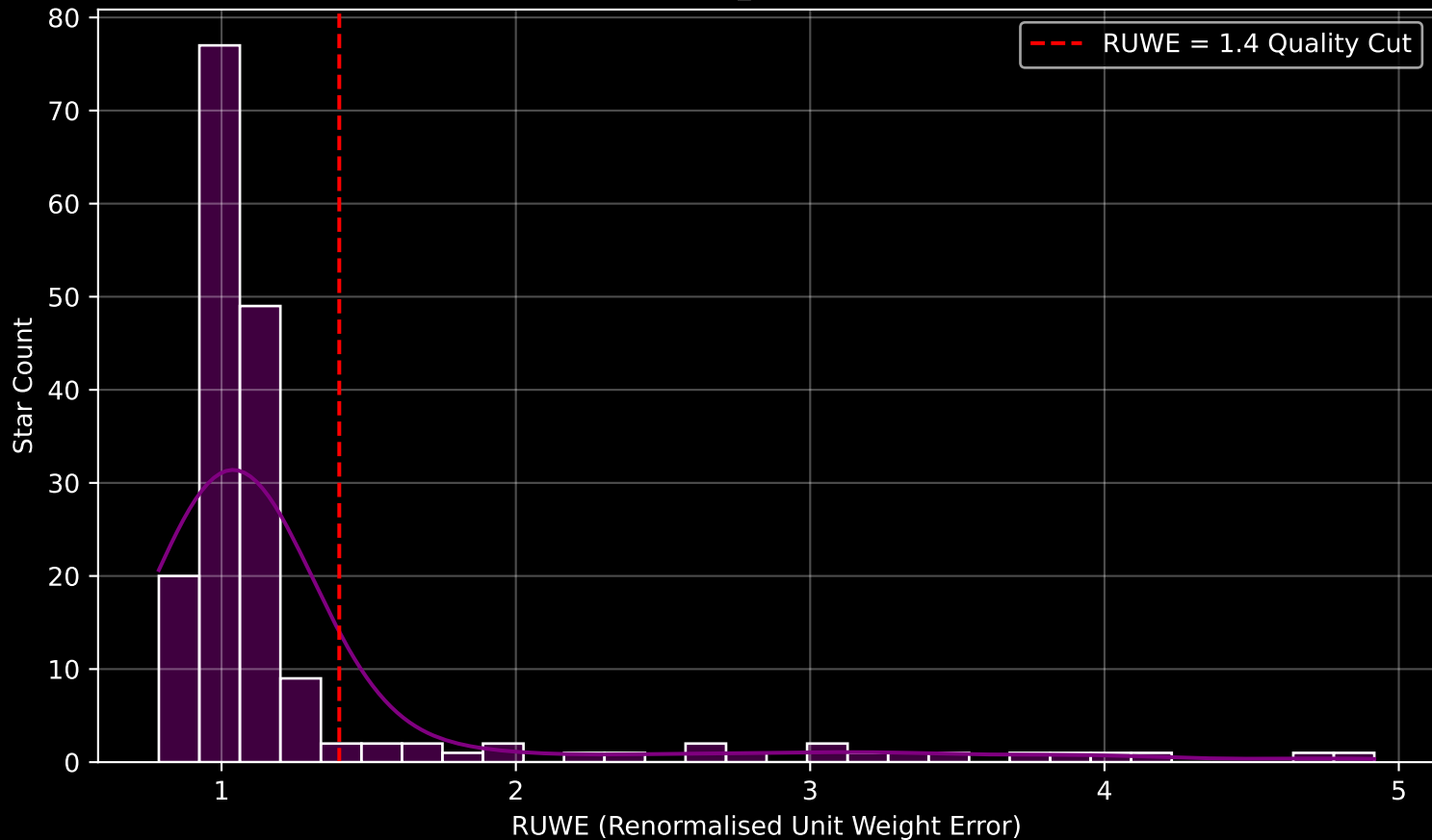
GAPOGEE DR17 Field [178+30_MGA] RUWE Distribution (n= 180)
