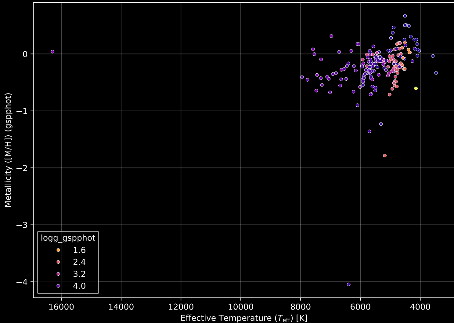
APOGEE DR17 Field: [178+30_MGA] Stellar Population Parameters (n= 193)
