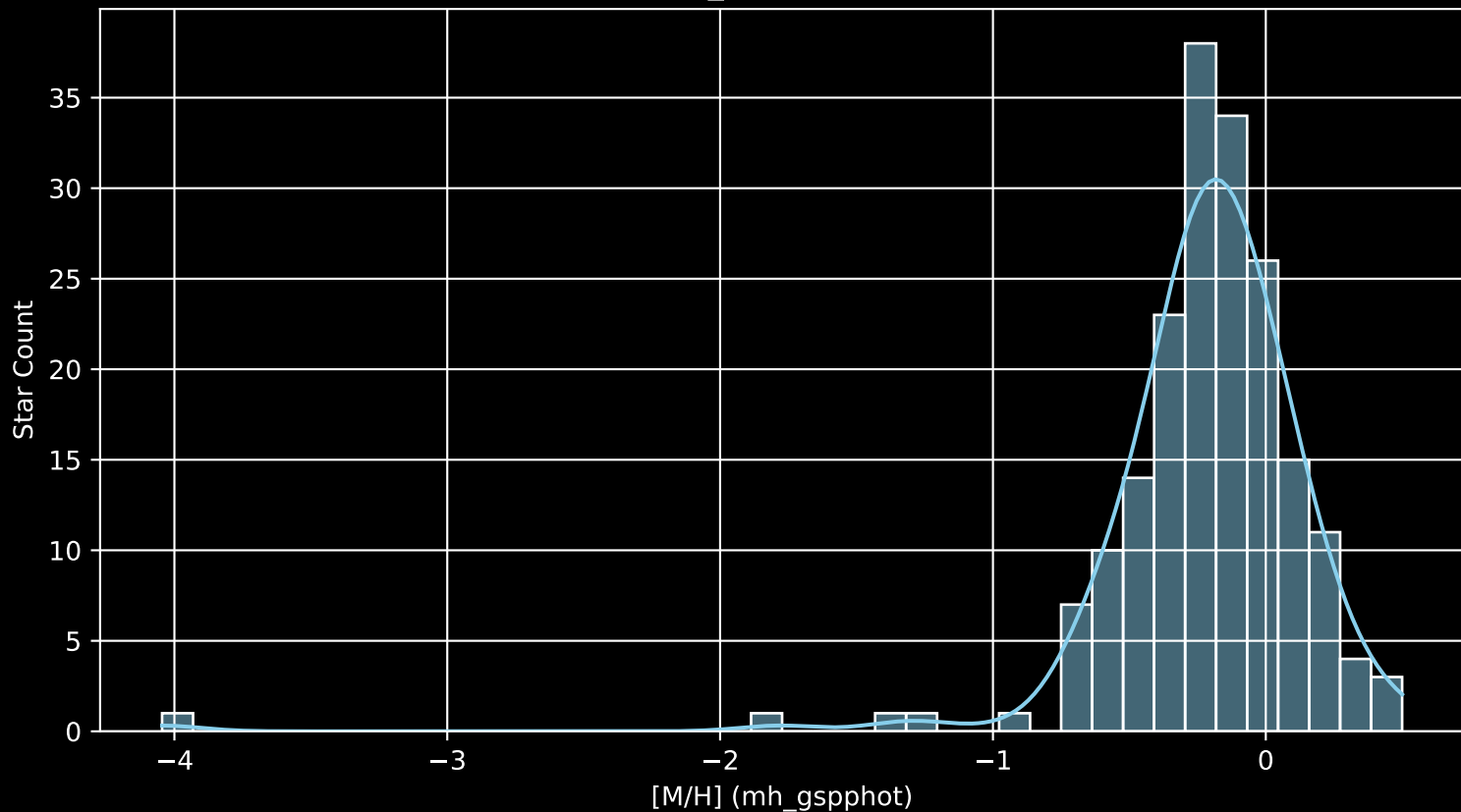
APOGEE DR17 Field: [178+30_MGA [M/H] (mh_gspphot) (n= 190)
