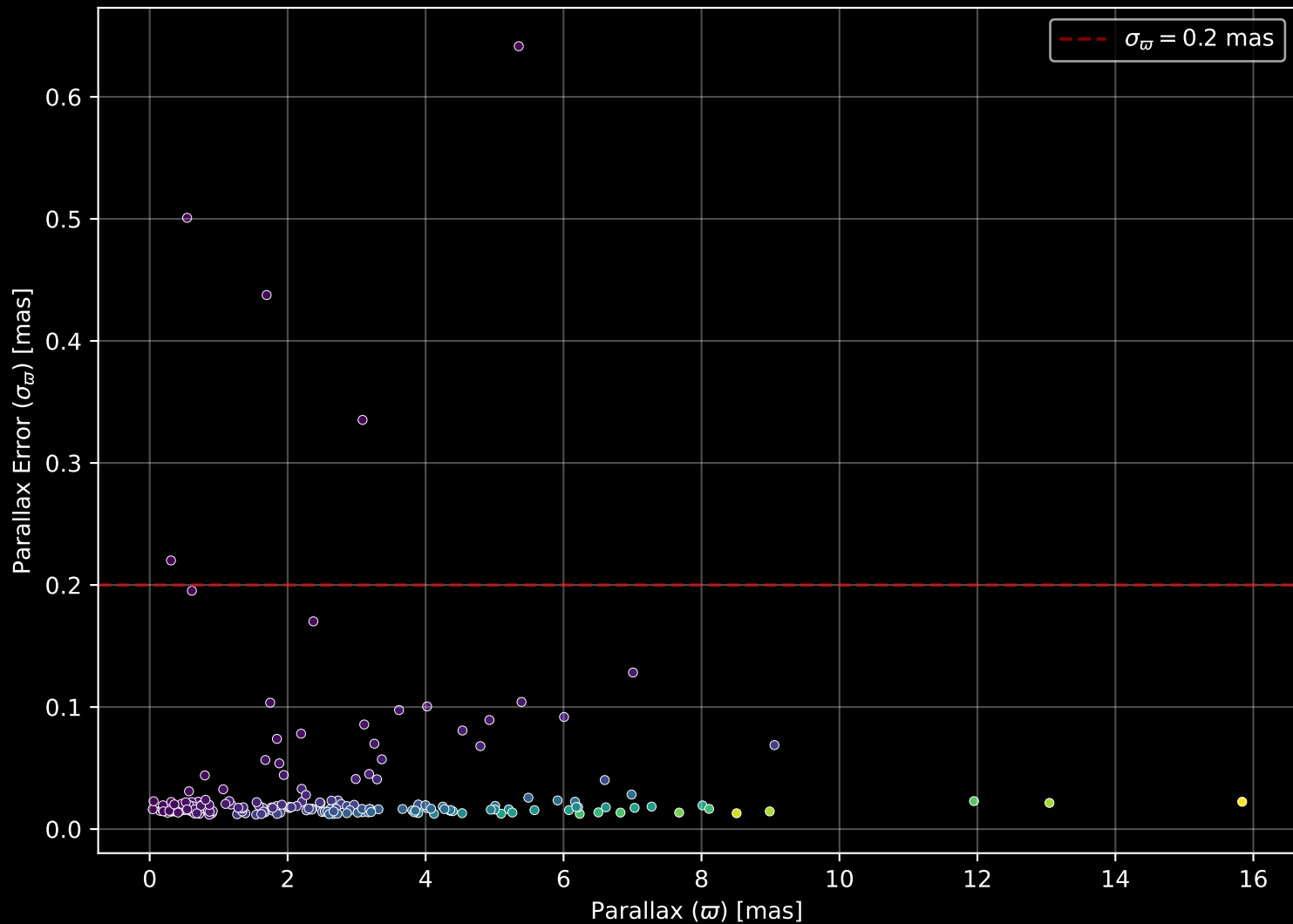
APOGEE DR17 Field: [178+30_MGA] Parallax Quality (n= 193)
