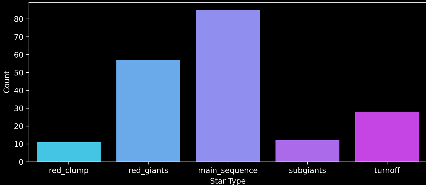
APOGEE DR17 Field: [178+30_MGA] Count plot of Star Type
