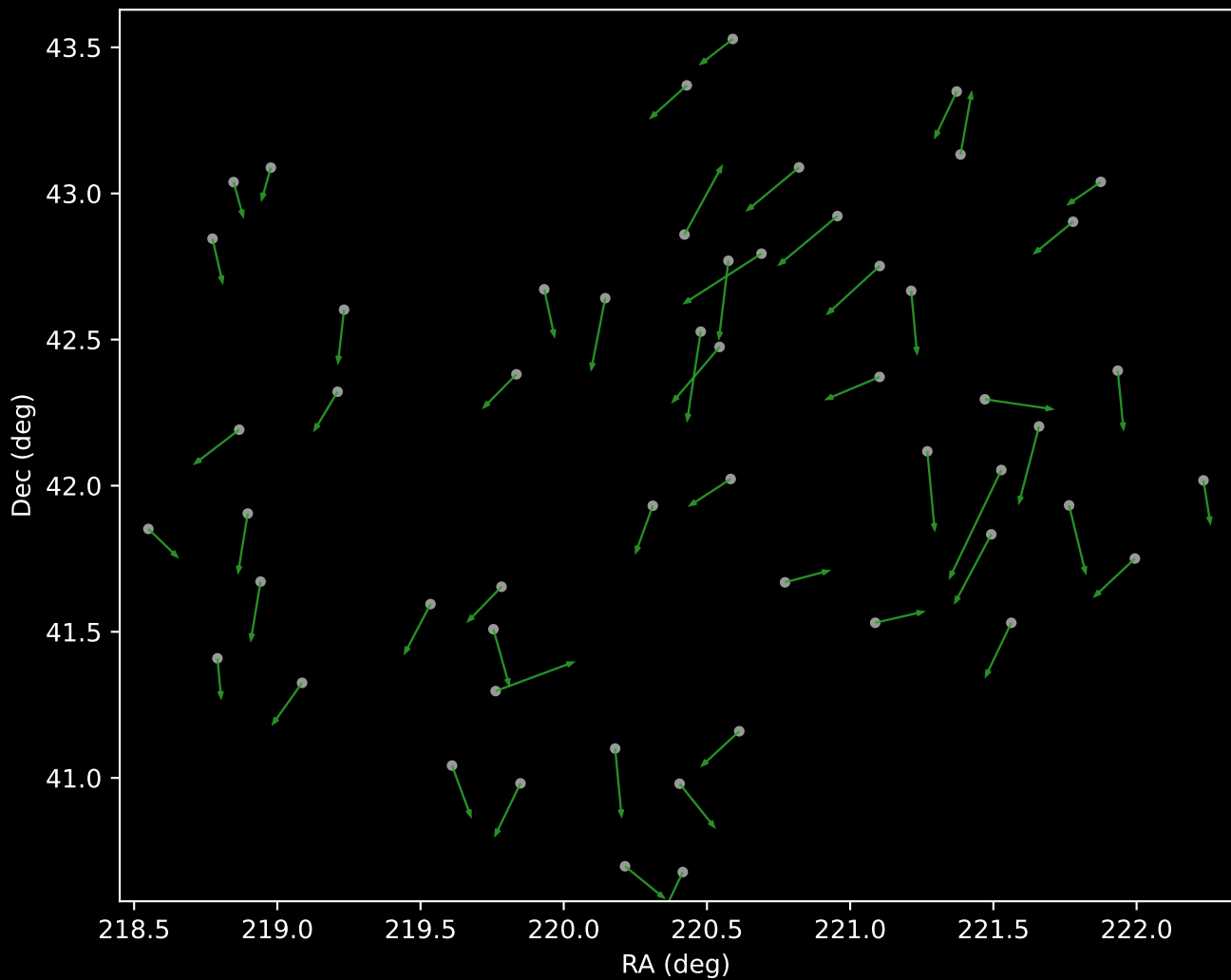
APOGEE DR17 Cluster 4 Proper Motion Vectors (n=55)
