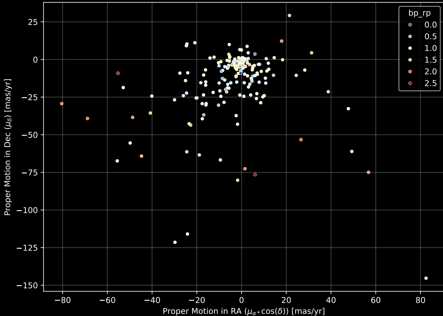
APOGEE DR17 Field: [178+30_MGA] Proper Motion Diagram (n= 193)
